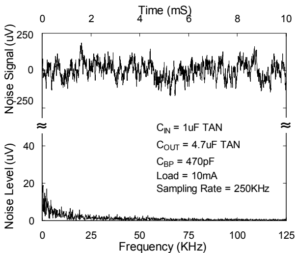
Noise Signal & Spectrum Distribution
