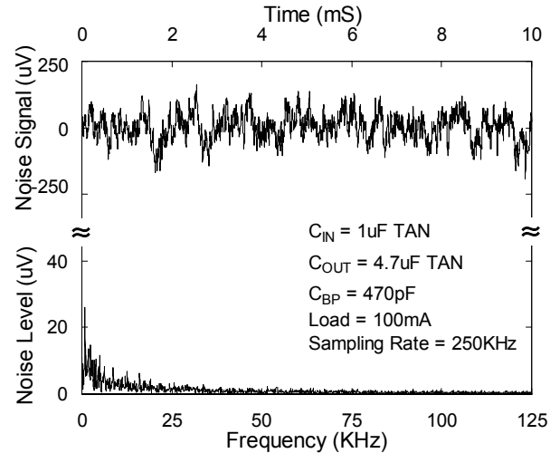
Noise Signal & Spectrum Distribution
